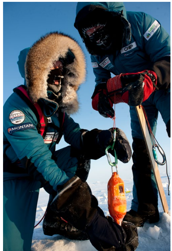
The SonTek CastAway-CTD is so compact it can be kept warm before deployment by simply tucking it inside the explorer's jacket.
